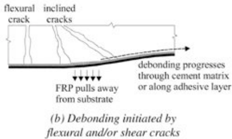
From ACI 440.2R-08
